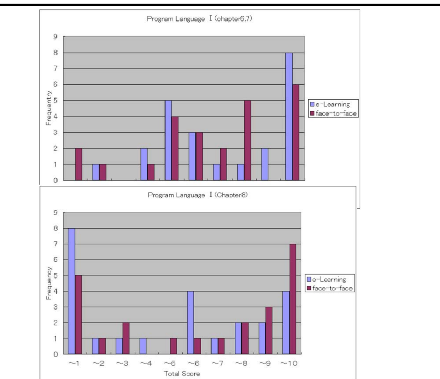
The comparison of score distribution in e-learning and face-to-face
