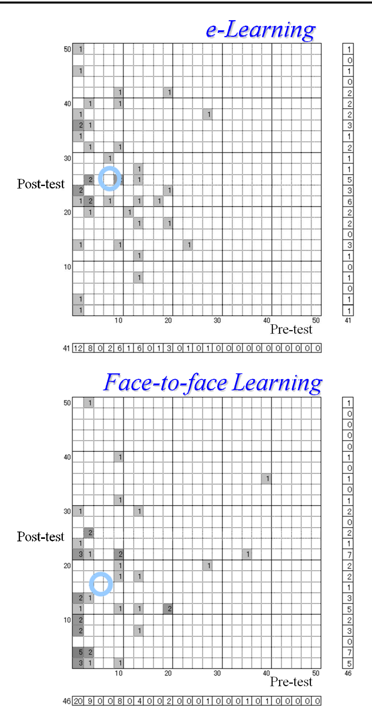
The score distribution on the pre-test and post-test
